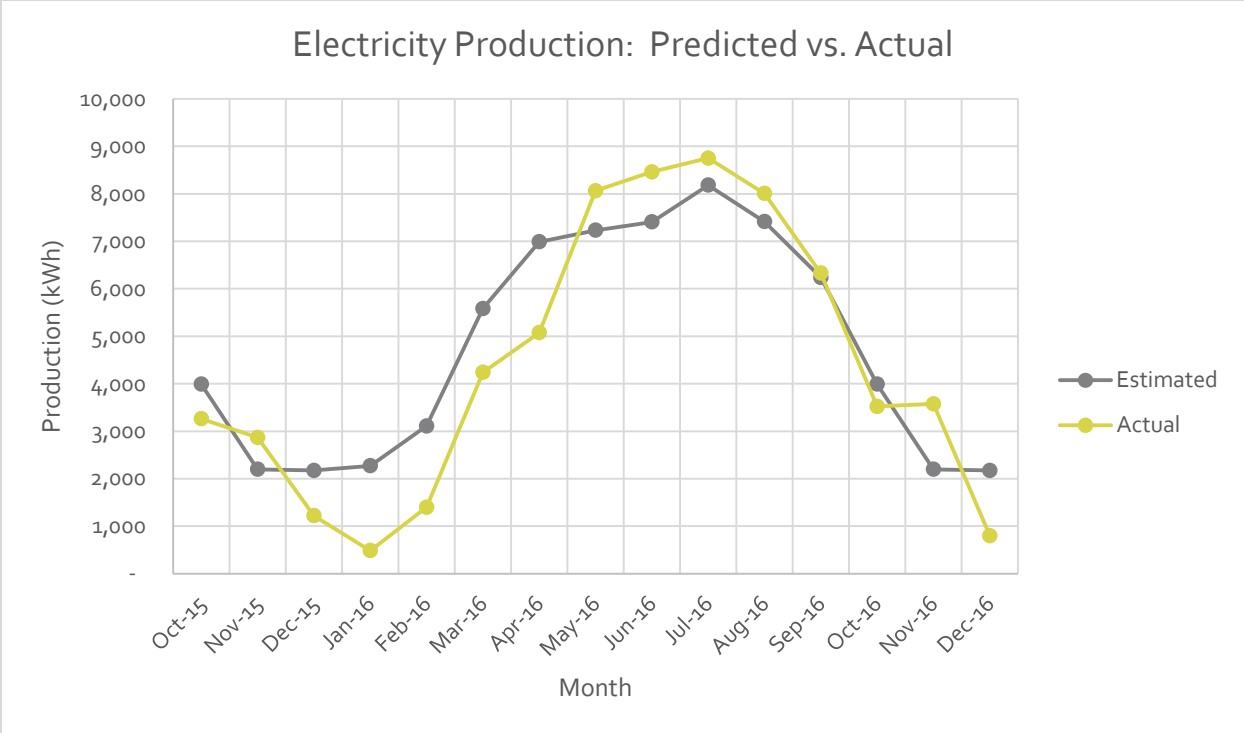
Figure 2 - Electricity produced by the King Orchards solar energy system since implementation compared to predicted values provided by Harvest Energy Solutions.
